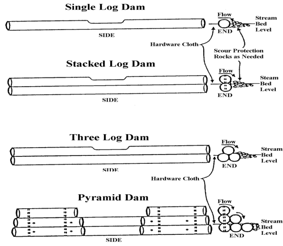
LOG DROP STRUCTURE DETAILS No Scale
