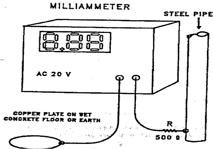
Figure 3, Set Up for Measuring Current Cow Contact Point to Ground (3-31-22)
