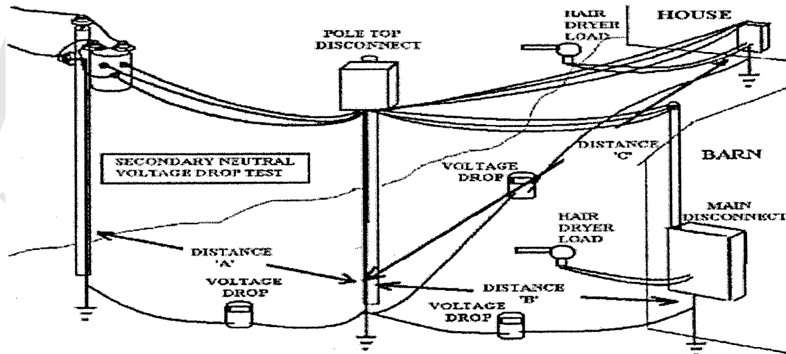
Figure 5, Secondary Neutral Voltage Drop Test Arrangement. (3-31-22)
