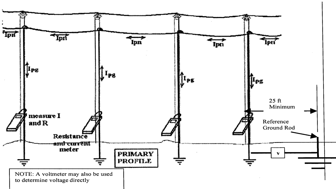
Figure 4, Primary Profile Test (3-31-22)
