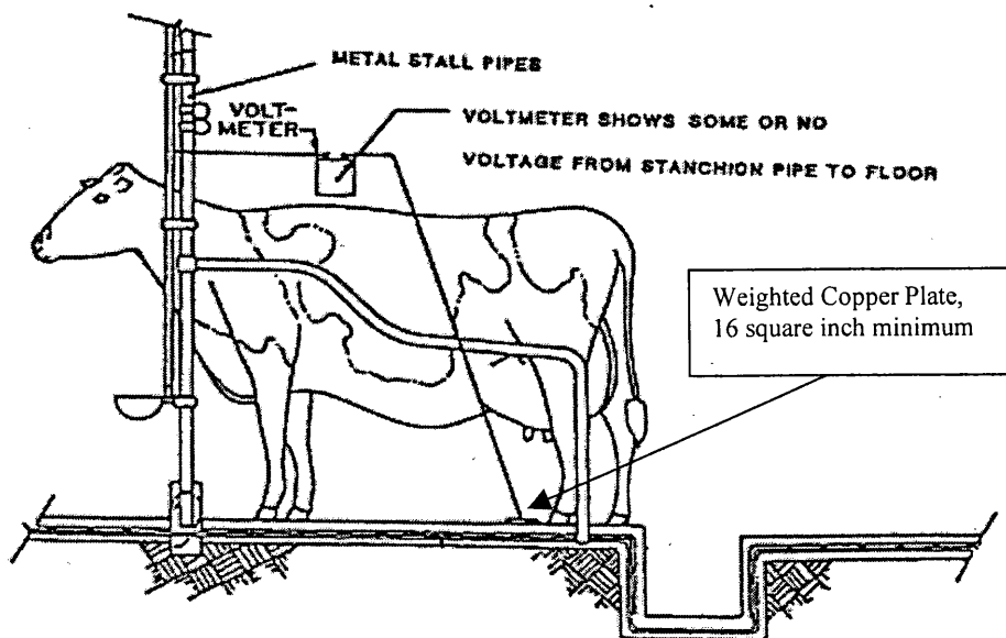
Figure 1, Cow Contact Test. (3-31-22)
