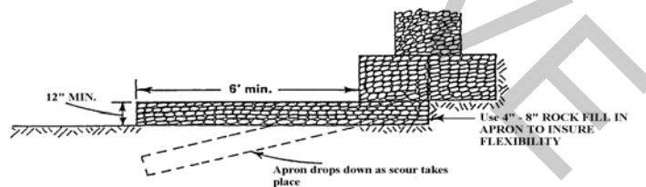
FIGURE 6. Placement of mattress toe protection
