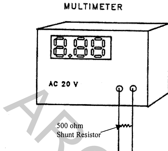
Figure 2, Cow Contact Voltage Measurement.
