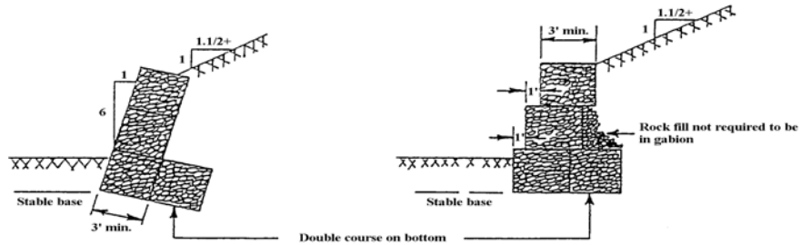
FIGURE 5. Retaining wall construction
