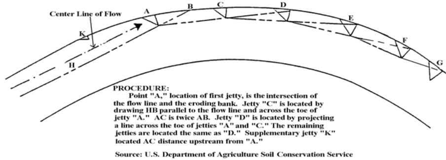
FIGURE 15. Method of Locating Jetties
