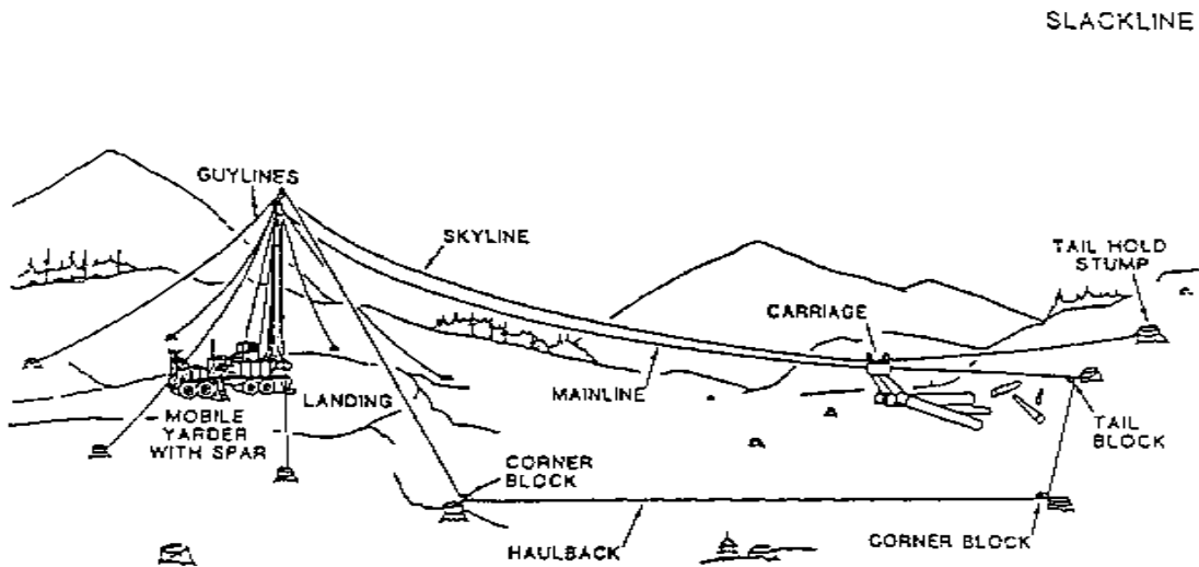
FIGURE 013.01-G SLACKLINE
