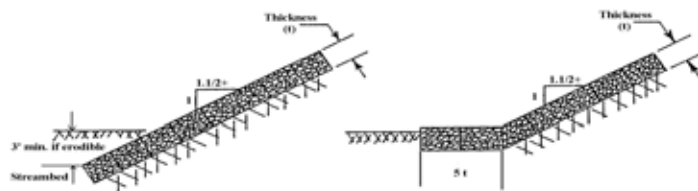
FIGURE 4. Mattress Construction
