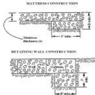
FIGURE 7. Mattress construction - views show cross-sections at end of gabion section looking down along the slope of the channel
