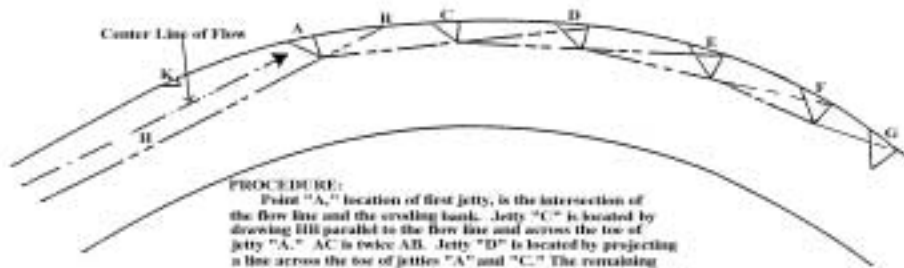
FIGURE 15. Method of Locating Jetties
