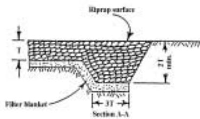
View shown above is cross section at end of riprap looking down along the slope toward streambed.
