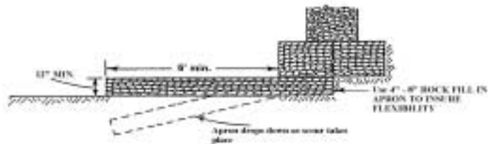
FIGURE 6. Placement of mattress for protection
