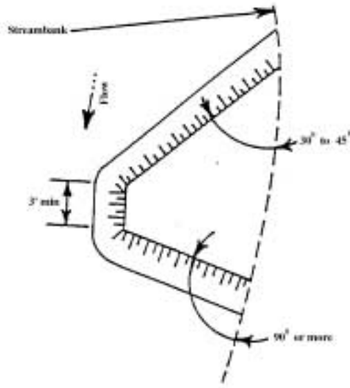
FIGURE 16. Jetty Height in Relation to Streamflow Depth
