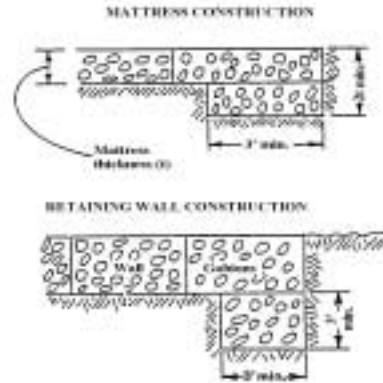
FIGURE 7. Mattress and retaining walls are cross sections at end of gabion section looking down along the side slope of the channel
