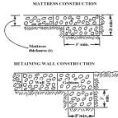
FIGURE 7. Minimum details - views shown are cross-sections at end of gabion section looking down along the side slope of the channel
