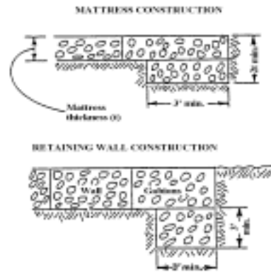
FIGURE 7. Minimum cutoffs - views shows are cross-sections at end of gabion section looking down along the side slope of the channel
