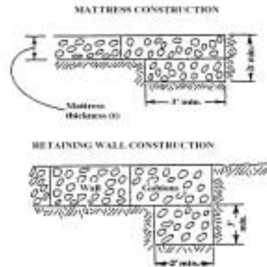
FIGURE 7. Minimum setbacks - views shown are cross-sections at end of gabion section looking down along the side slope of the channel
