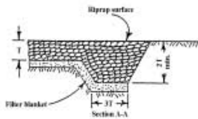
FIGURE J. Protection against undermining
