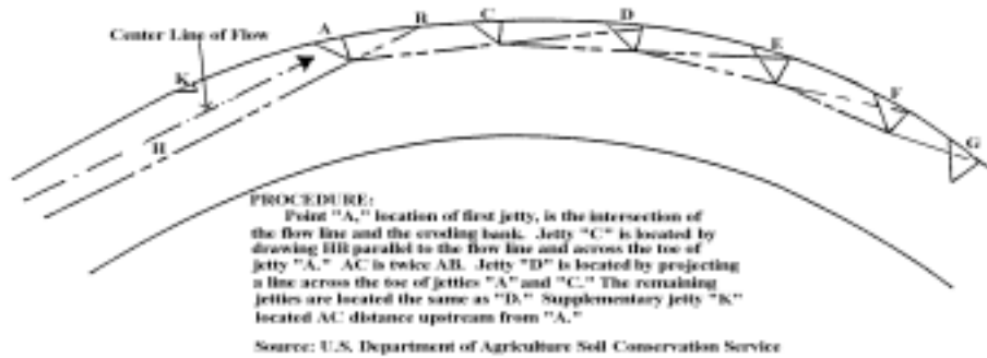
FIGURE 15. Method of Locating Jetties
