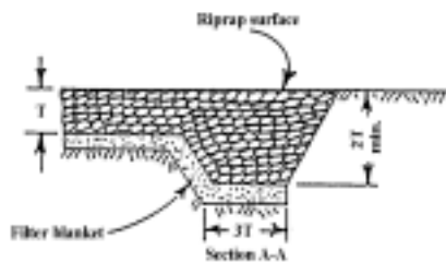
View shown above is cross section at end of riprap looking down along the slope toward streambed.
