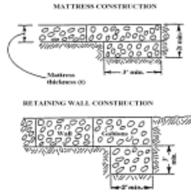
FIGURE 7. Minimum cutoffs - views shown are cross-sections at end of gabion section looking down along the slope of the channel
