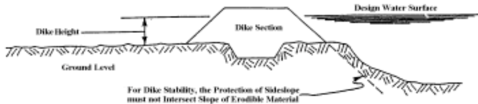
FIGURE 12. Dike Cross-Section
