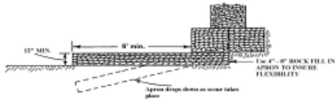
FIGURE 6. Placement of mattress for protection
