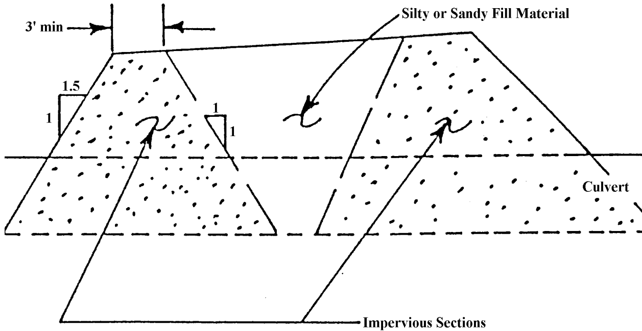
FIGURE 19. Culvert Backfill Using Silty or Sandy Material
