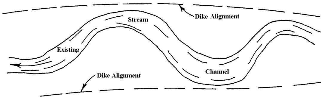
FIGURE 13. Desirable Dike Location
