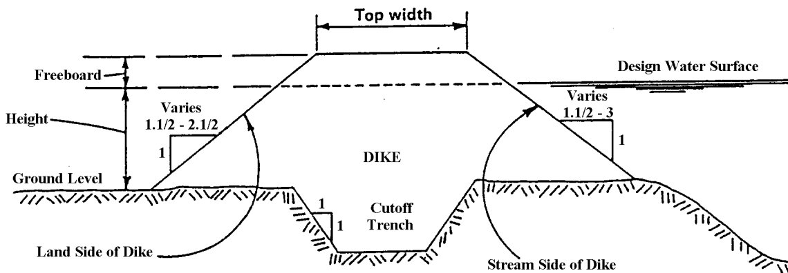
FIGURE 14. Minimum Criteria for Dike or Levee Cross-Section
