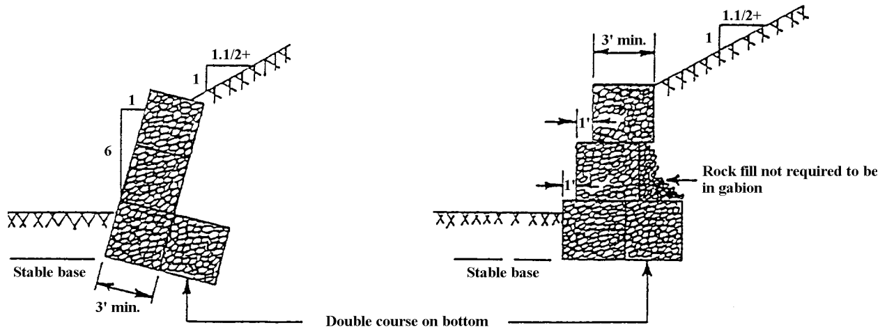
FIGURE 5. Retaining wall construction
