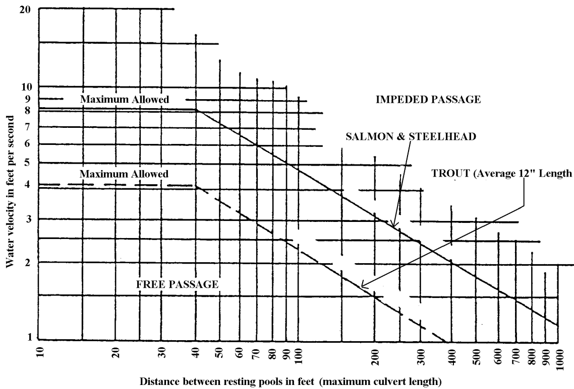
FIGURE 17. Swimming capability of migrating salmon and trout (Alaskan Curve)
