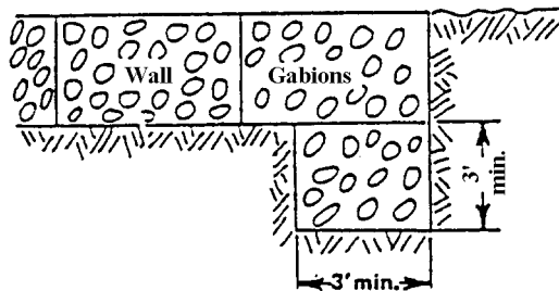
FIGURE 7. Minimum cutoffs - views shown are cross-sections at end of gabion section looking down along the sideslope of the channel
