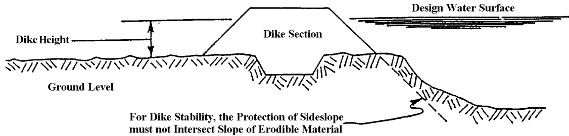
FIGURE 12. Dike Cross-Section
