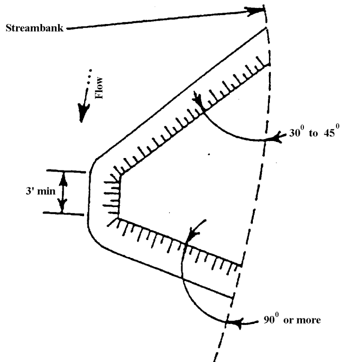
FIGURE 16. Jetty Height in Relation to Streamflow Depth
