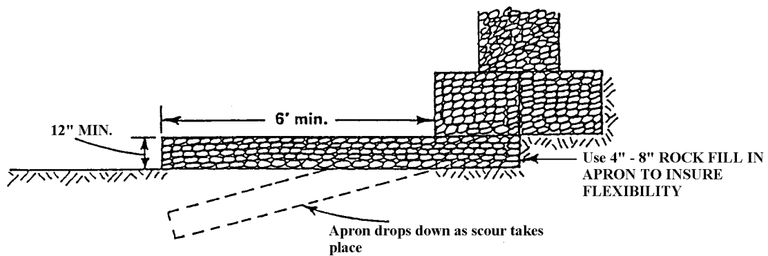
FIGURE 6. Placement of mattress toe protection
