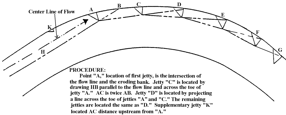
FIGURE 15. Method of Locating Jetties
