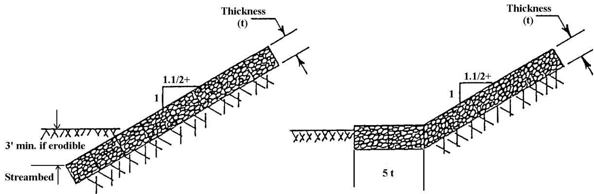
FIGURE 4. Mattress Construction
