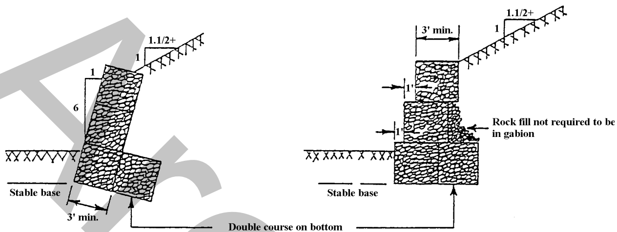
FIGURE 5. Retaining wall construction
